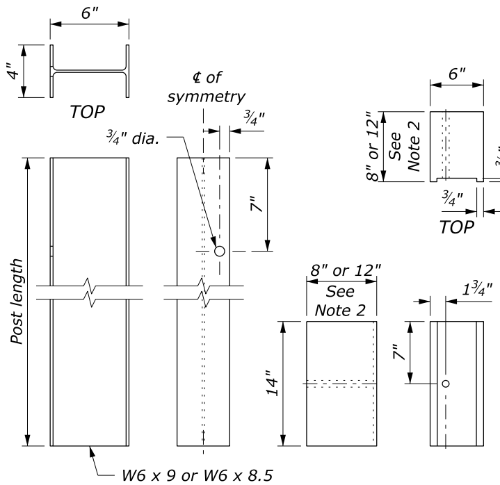
STRUCTURAL SHAPE POST BLOCKOUT POST FACE
