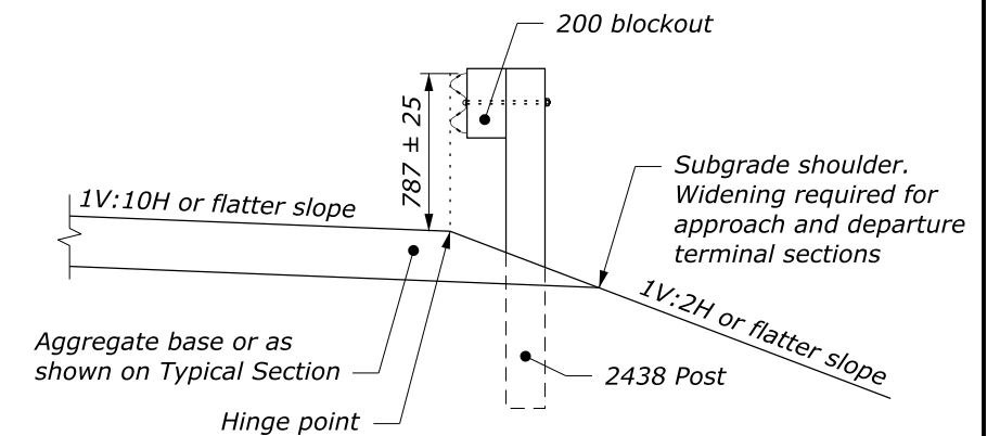
TYPICAL GUARDRAIL CROSS SECTION 2438 POST ON SLOPE, 200 BLOCKOUT
