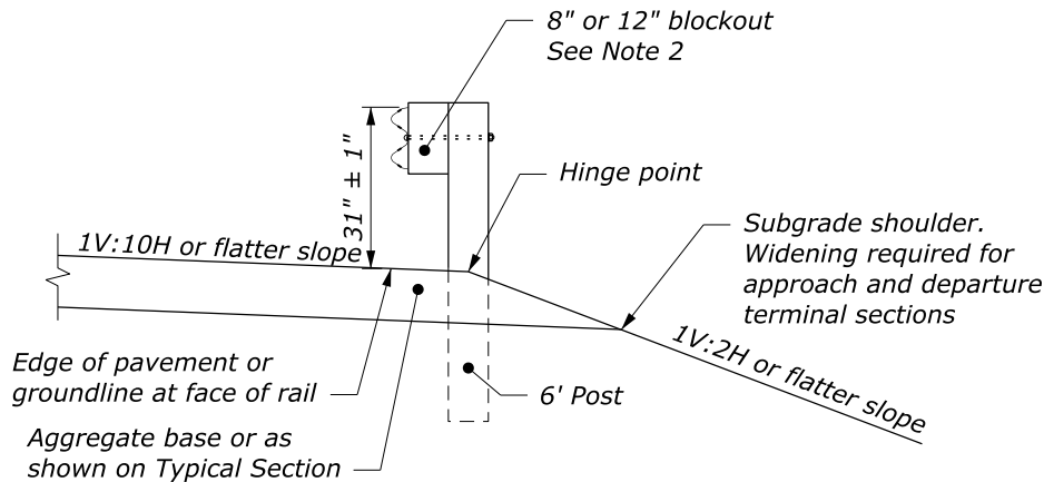
STRUCTURAL SHAPE POST BLOCKOUT POST FACE
