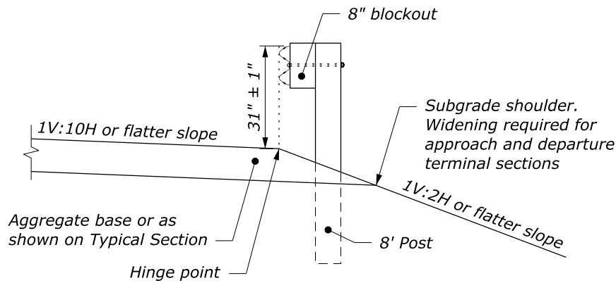
TYPICAL GUARDRAIL CROSS SECTION 8' POST ON SLOPE, 8" BLOCKOUT
