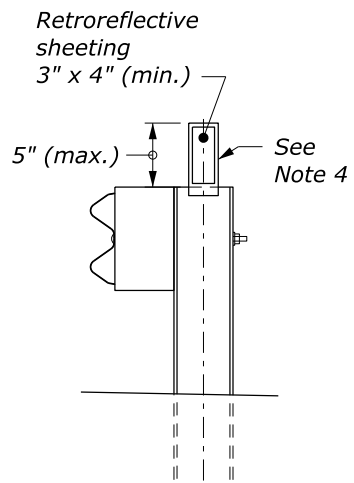
FLEXIBLE DELINEATOR GUARDRAIL MOUNT
