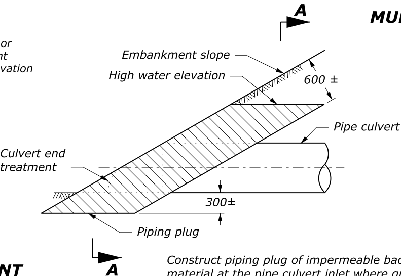
PIPING PLUG
