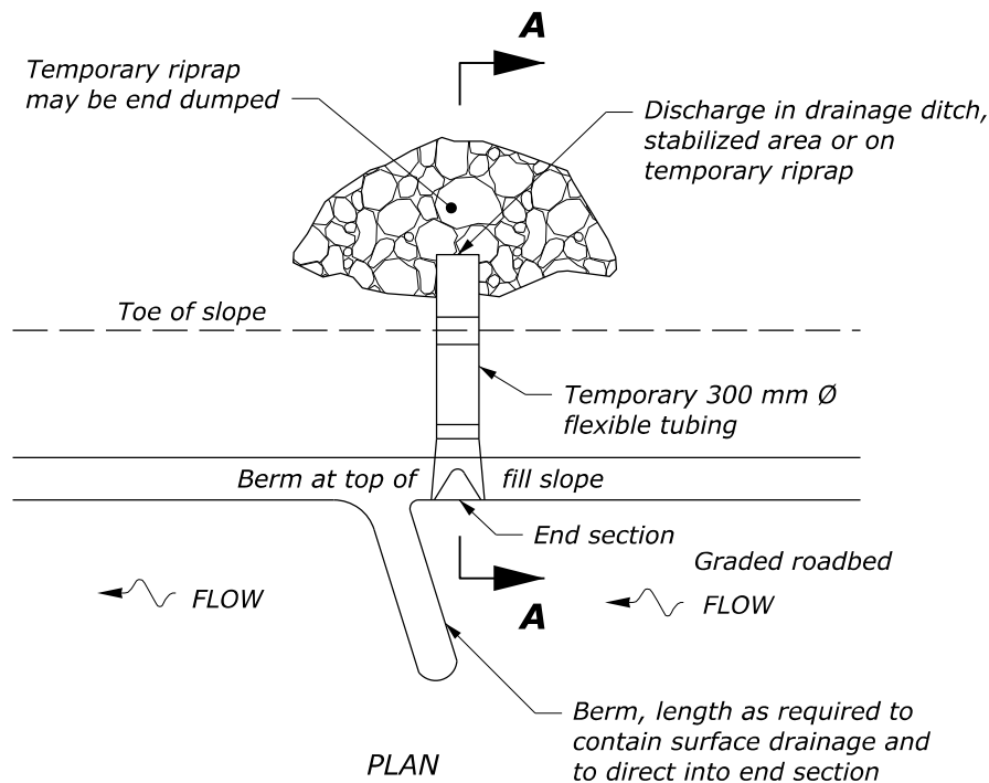
SLOPE DRAINS
